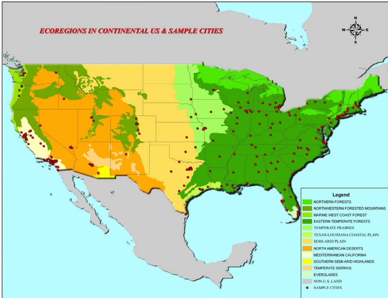
Figure 1 Ecoregions of selected cities in Continental US
